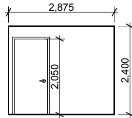
5 INTERIOR ELEVATION - LOOKING EAST
