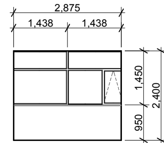
4 INTERIOR ELEVATION - LOOKING WEST
